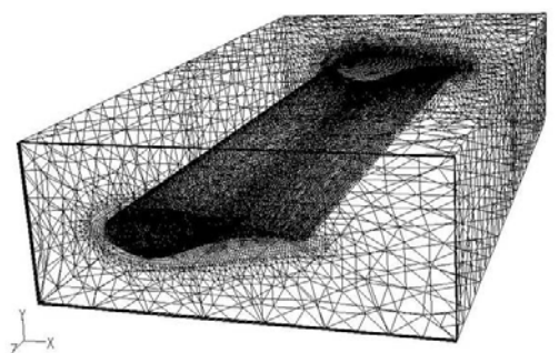
Grid FLUENT 6.0 (3d, dp, segregated, lam) Jun 30, 2004
