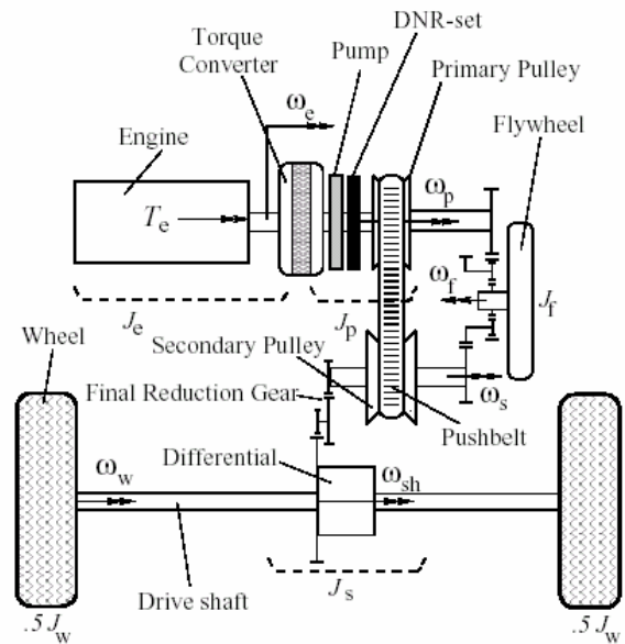
Gambar 3. Model Powertrain
