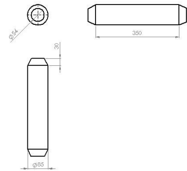
Gambar 3.5 Dimensi resonator
