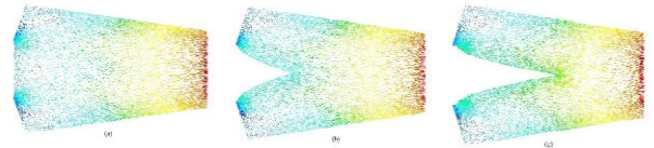
Gambar 3.4. Simulasi velocity (a) Kolektor tanpa spike (b) Kolektor spike 50 mm (c) Kolektor spike 100 mm
